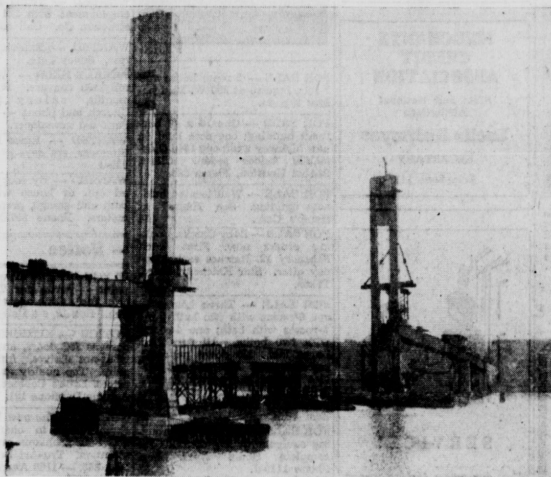
ALLEY OOP!—Barges floated this 330-foot section of the new pedestrian bridge into place across New York's Harlem River to Ward's Island. It was then hoisted into place to complete the 950-foot-long bridge which will make another park area available to nearby residents.
