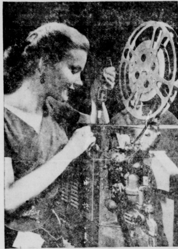
BRIGHT LIGHT—A lamp, one-eighth as bright as the sun, has been developed to lend to televised motion pictures the quality of live telecasts. Actress Ava Norring shows in Bloomfield, N. J., how the new mercury vapor lamp slides into a movie projector. The lamp can also be used in searchlights where accurate cloud ceiling measurements are needed. The 800-watt light source can bounce a beam off a cloud 2½ miles high.
