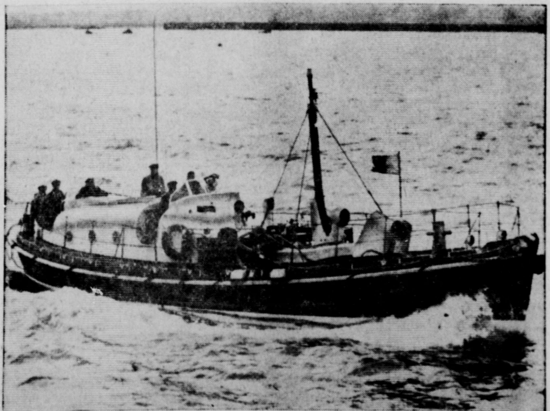
IT'S THE BEST —Going through a trial run at Southampton, England, is the world's most modern lifeboat, the Sir Godfrey Baring, which will be shown at the 1951 Festival of Britain before being assigned to rescue work in the North Sea. The craft features aluminum alloy superstructure, jets for squirting oil on rough seas, and pressure cookers to provide hot food.
