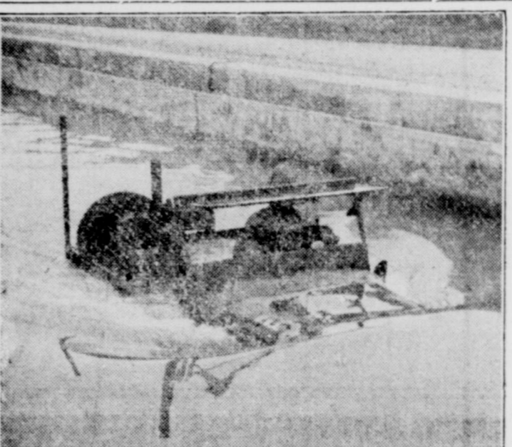
BATH FOR WATER-PROOF ARMY JEEP—At Aberdeen Proving Ground this jeep is tested under water. Its engine is waterproofed. Two pipes, one at the windshield and the other at the rear of the vehicle, are breather and exhausts. While submerged the ignition may be turned off and the motor restarted. The driver is equipped with a rubberized suit. (Official Department of Defense photo).
