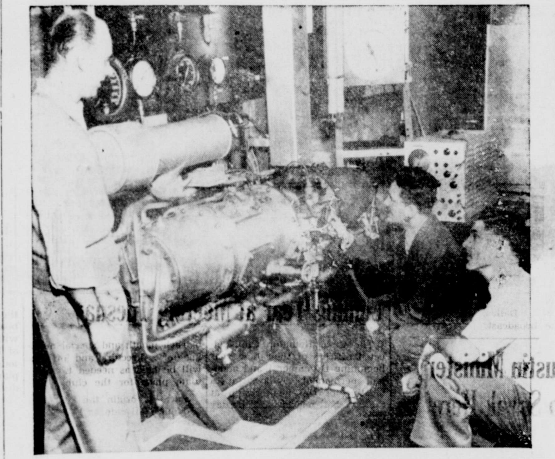
STUDY GERMAN DIESEL—This German-developed "free piston" Diesel may give engineers answers to the problem of how to develop a turbine engine for automobiles. The model being studied here in a Stanford University laboratory, in California, is an air compressor, but the engine can also be designed as a power gas generator for a turbine.
