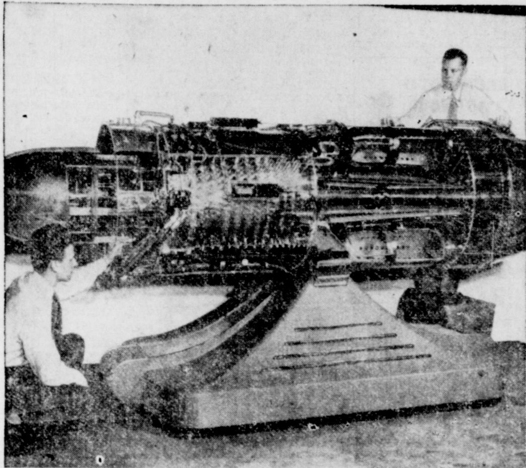
JET ENGINE DISPLAYED —By means of this jet engine, internal operation of the J-47 turbojet which powers the Air Force's largest and fastest jet planes is demonstrated publicly in Cleveland O., for the first time. The engine is cut away to show the movements of its internal parts, but its performance never has been disclosed except in general terms.
