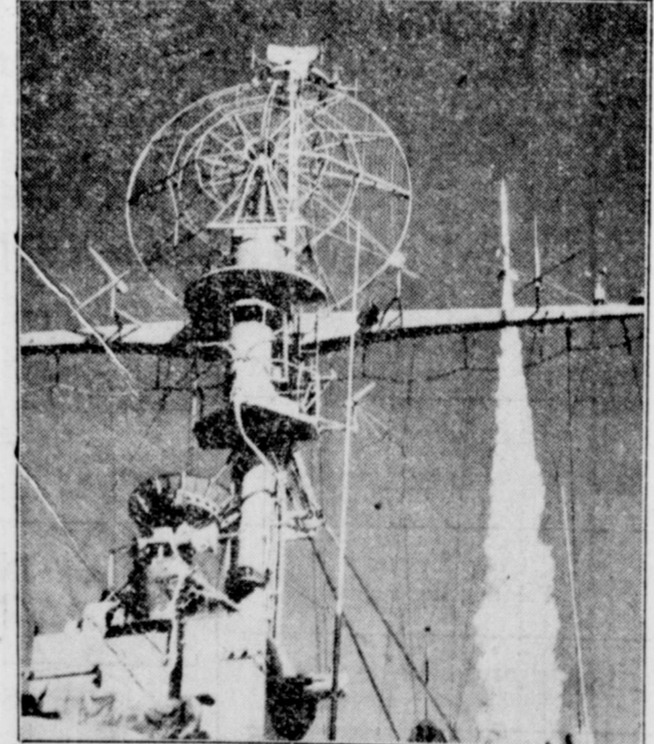
OUT OF THIS WORLD—The elaborately wired instrument is the radar antenna above the deck of the USS Norton Sound, and shooting skyward, leaving a trail of white vapor, is the Navy's aerobee sounding rocket used in the study of cosmic ray intensity. The rockets, fired at a point approximately 700 miles off the west coast of South America, attained an altitude of more than 65 miles above the ocean. Cosmic ray data is obtained from instruments in the nose of the rockets.
