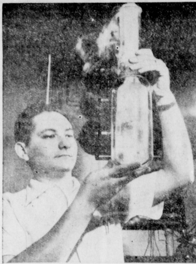
BOILING COLD —Dr. Aaron Wexler drops solid chunks of air, with a temperature of 340 degrees below zero, into a flash of liquid helium in Pittsburgh, Pa. Because the frozen air is "hotter" than the liquid helium, it causes the latter to "boil" and overflow the mouth of the flask in billows of foam.
