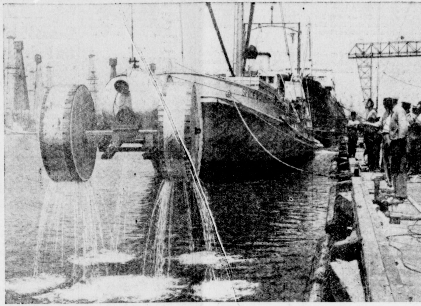
NEW EXPLORING METHOD —This 7000-pound Benthoscope is hauled from the Long Beach, Calif. harbor after a 340-foot test dive was made by Dr. Otis Barton of New York. Barton plans to drop from 1500 to 1800 feet into the Pacific Ocean to study life in those depths. The three cable-drum wheels enable the 'scope to be dragged along the bottom.
