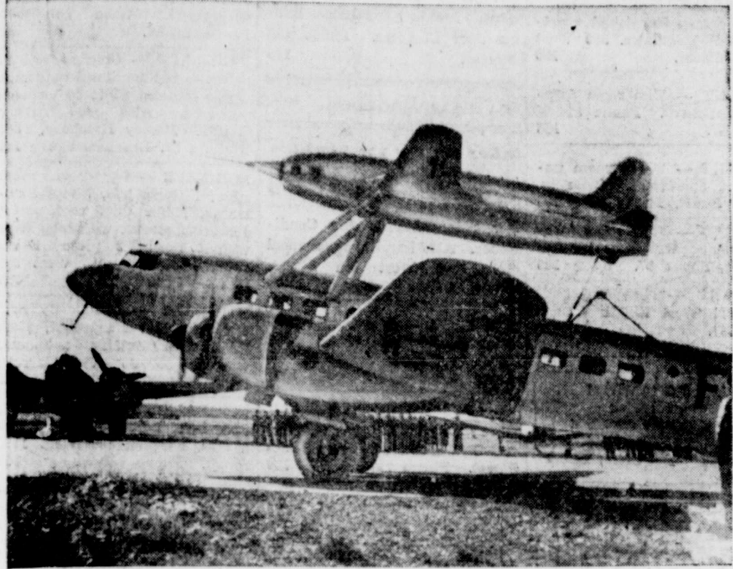
TEST NEW FRENCH JET PLANE —This latest French jet plane, called Composite Leduc, is being tested at Toulouse. The jet is carried atop a standard plane, and at a high altitude it takes off from it with jet power. The Leduc may reach supersonic speed.
