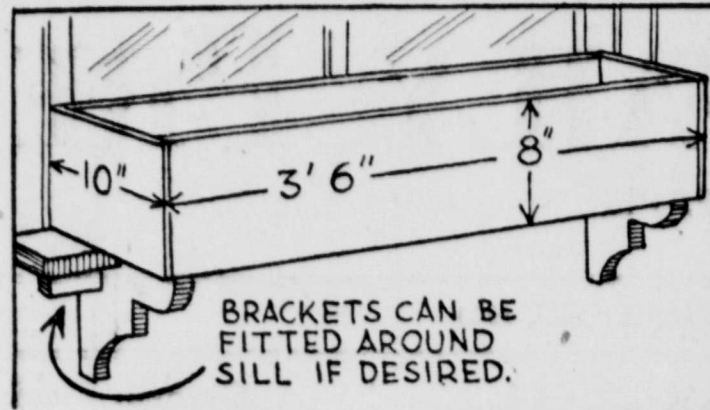
Working Drawing for Standard Window Box.
