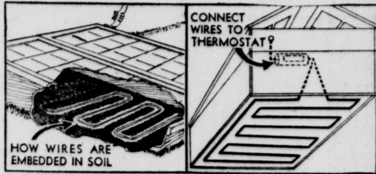
How to Install Electric Heating Cable With Thermostat in Hotbed.
