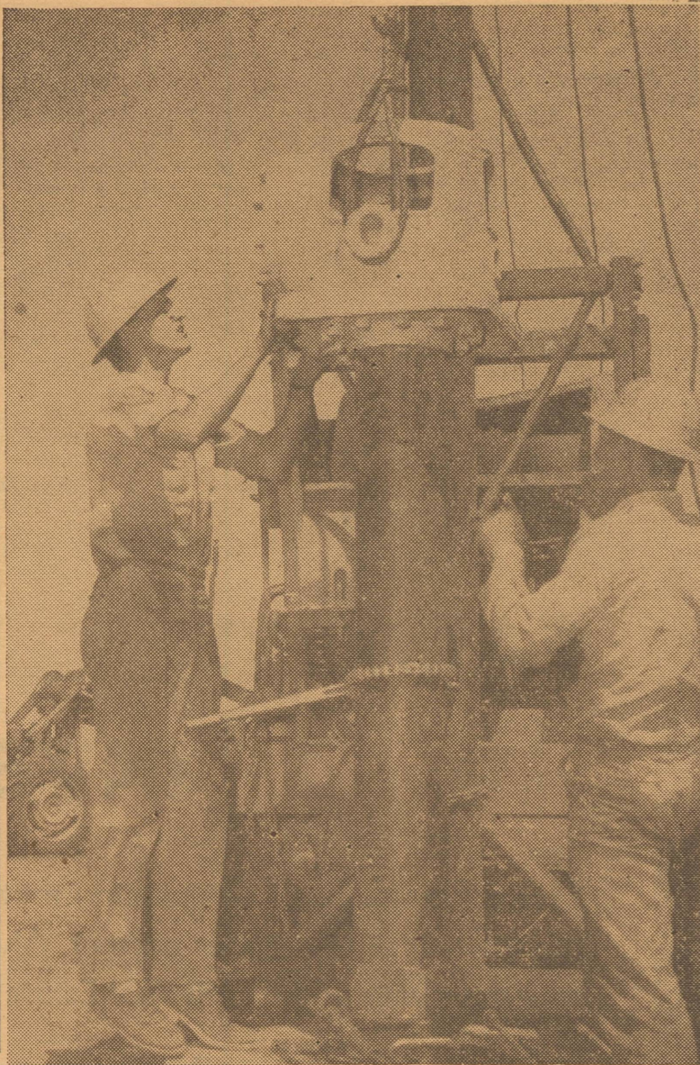
STEADY DOES IT —Johnnie Parker and Frank Reeve of Parmer County Pump Company ease the last joint of pipe into the city's new well at the cemetery. Atop this joint is the familiar pump base. This well was drilled 470 feet deep. Drilling started Thursday, and this picture was made Saturday afternoon. Development started.
