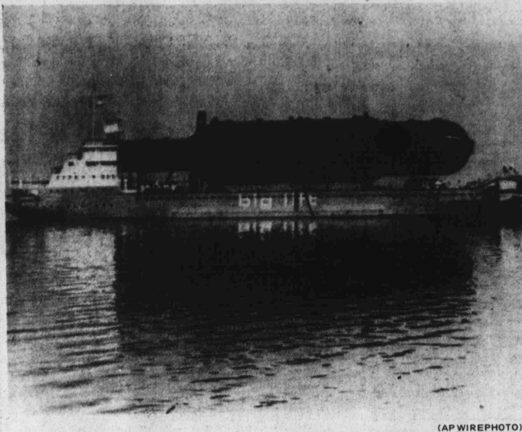
PIGGY-BACK TOWER — A 615-ton, 200-foot long distillation tower arrives at Exxon's Baytown refinery near Houston. It is the largest tower in an expansion program at the refinery that is scheduled to be completed in late 1976. The refinery's capacity will be increased from its present 400,000 barrels per day to approximately 650,000 barrels daily making it the largest refinery in the world.
