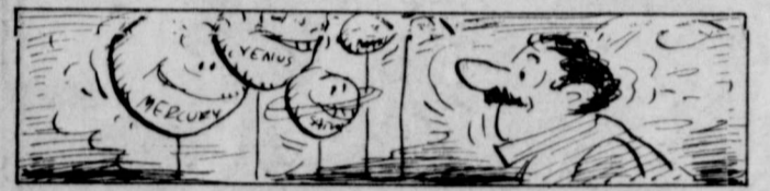
Five planets are visible to the naked eye: Mercury, Venus, Mars, Jupiter and Saturn.
