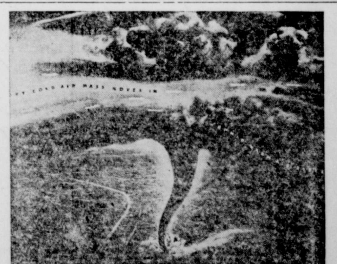
BIRTH OF A TORNADO occurs when a cold and a warm air mass collide, and the heavier cold air is deflected above the lighter warm air. In this topsy-turvy situation, a tongue of cold air dips into the warm air, which in turn moves upward to fill the void thus created.
