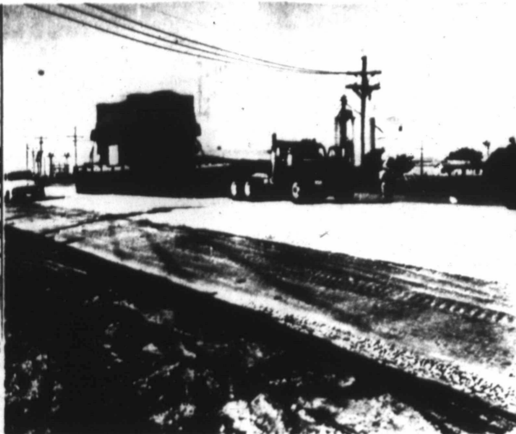
MOVING 269 TONS - You don't just toss 538,000 pounds of generator into the back of a pickup and tear out with it. It took nearly 12 hours to move this big unit from the railway station at Amherst to Plant X last Friday. In the photo at left, the generator is already loaded and the unit is attempting the turn from the railway depot onto the
