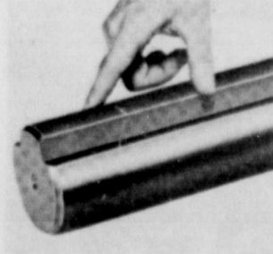
3 1/2" Axles: Extra large diameter for extra strength. Built-up integral axle key does away with key grooves.
