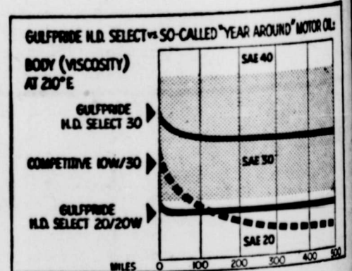
See how Gulfpride H.D. Select holds its "body" (viscosity). This new oil contains no artificial thickeners that break down under heat and pressure. But note how quickly a typical multi-viscosity 10W-30 oil starts to lose its body.
