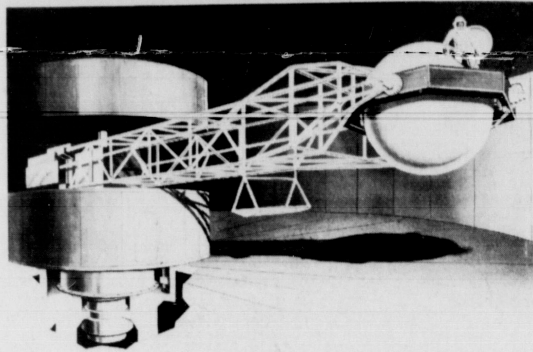
This is a drawing of the Timken bearing-equipped flight acceleration simulator whose main drive system was constructed by Westinghouse Electric Corporation for use by the National Aeronautics and Space Administration (NASA) in training astronauts for space travel.
