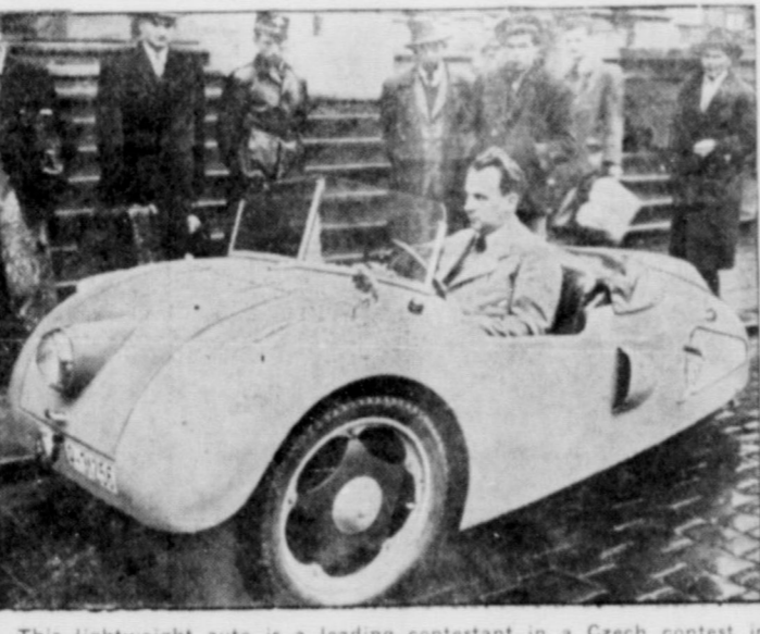
This lightweight auto is a leading contestant in a Czech contest in Prague to find a low-consumption, inexpensive car within the means of the average worker. Driven by a two-cylinder engine, located in the rear of the car, it has a maximum speed of 50 mph and travels 63 miles to a gallon of gas. It was built by a Prague office clerk in his spare time.
