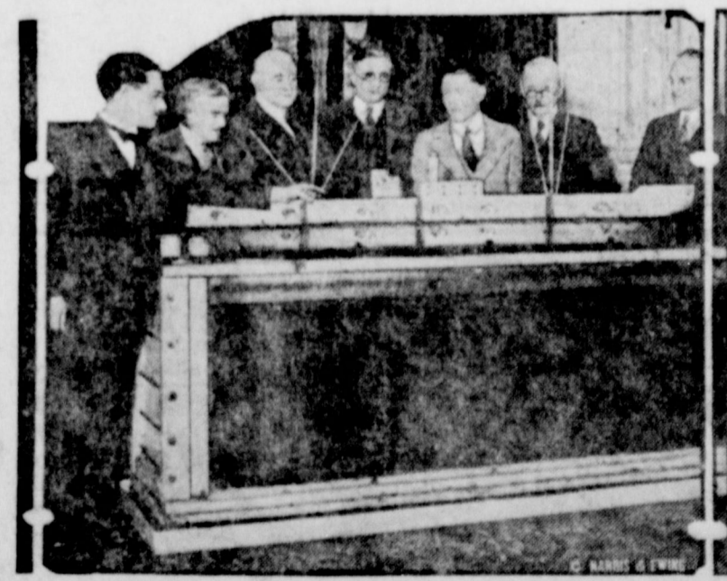
Adam T. Drekkolins of New York demonstrating to members of the naval affairs committee his invention which he claims will keep any ship from sinking, no matter how badly damaged. The invention is a collapsible chamber designed to imprison air in the hull of a disabled vessel. Even if a ship were completely filled with water, he claims the device would keep its upper deck above the surface, giving the crew a chance for their lives until rescuers arrive. Mr. Drekkolins is shown on the left in the photograph.
