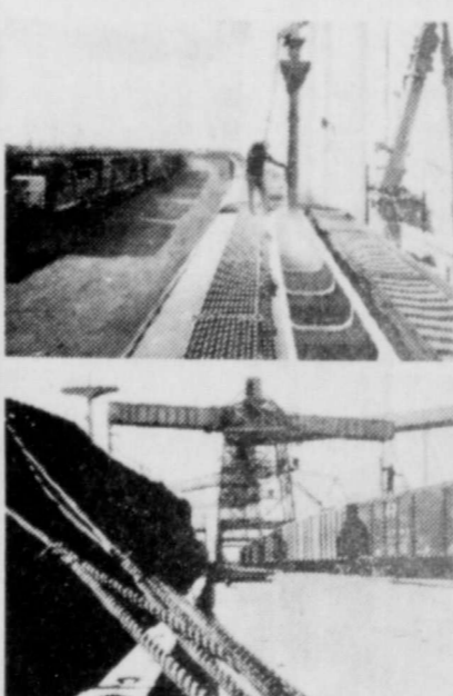
Trough hatches extending the length of car roof permit loading in about 12 minutes. Cars can be unloaded in less than three minutes.
