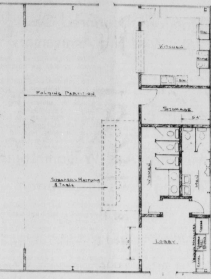
FLOOR PLAN MASSIE ACTIVITY CENTER, OVERALL SIZE 50' x 100'
