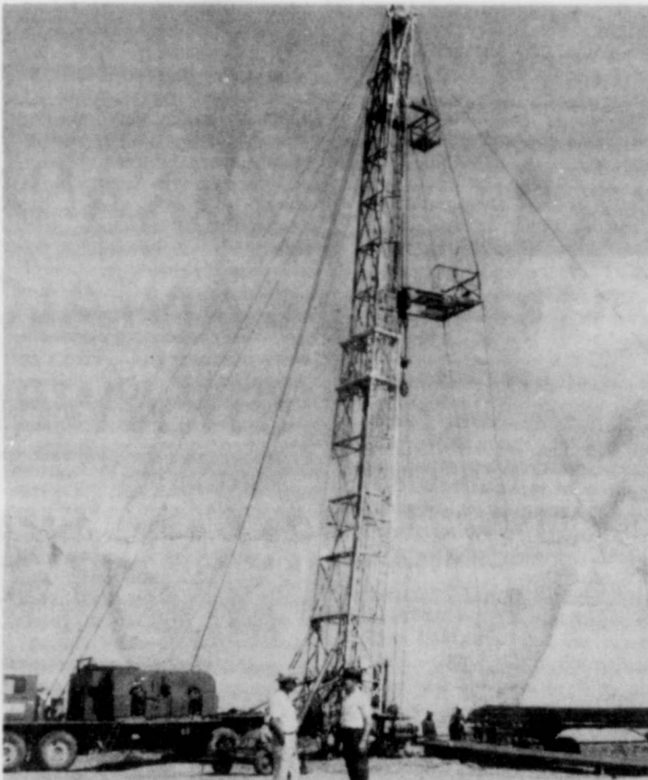
CASING AND PERFORATING RIG - goes to work on the oil well at the Fred Battey farm. In foreground is Doyle Moore and Battey. (Staff Photo)
