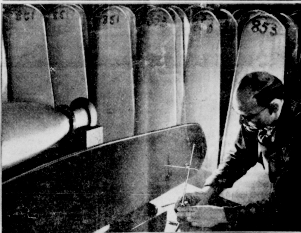
Careful inspection guarantees the quality of Chevrolet-produced war goods. Here a skilled metal worker makes the final inspection of aluminum propeller blade forgings, determines dead center in each blade, and measures to be certain that sufficient stock is included to allow for all machining operations.
