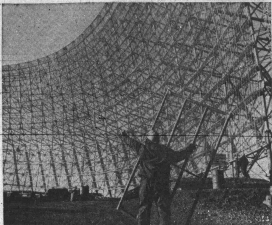
SETTING UP THE SCREEN — Workman carries steel frame, one of 2,000 used to build giant detection radar antenna at USAF base in Thule, Greenland. Antenna is one of four at Thule capable of detecting missiles 3,500 miles across the Arctic.
