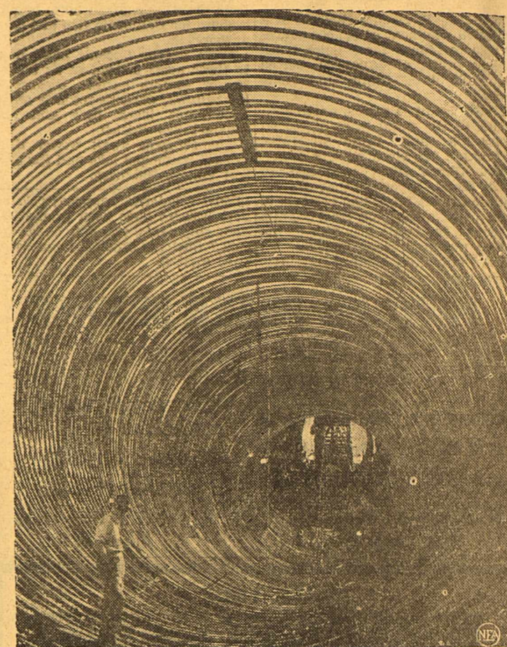
The "whatsit" picture above was taken inside the steel framework of a 4400-foot siphon on the Columbia Basin Project, Coulee Dam, Wash. It shows steel hoops, each 84 feet in diameter which will serve as ribs for a two-foot thick concrete shell.
