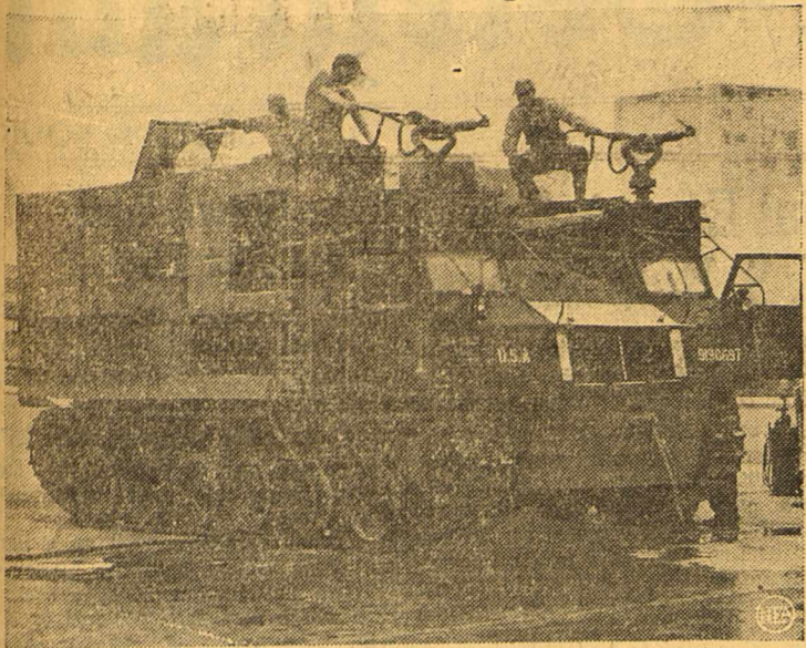
The modified M-8 cargo tractor pictured above was especially designed by the Air Materiel Command, Wright Field, Ohio, to combat airplane crash fires in Arctic weather. It was shipped to Ladd Field, Alaska, by cargo plane. An upper section, weighing 12 tons and looking like a small boxcar, houses the fire-fighting equipment. A tank holds 1000 gallons of water and 100 gallons of foam solution. It carries a crew of six.
