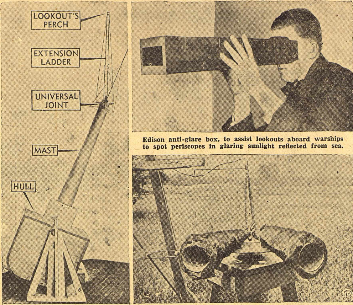
Edison anti-glare box, to assist lookouts aboard warships to spot periscopes in glaring sunlight reflected from sea. Extension ladder, to increase area of observation could be run up 87 feet above top of mast and remain vertical despite ship's roll. Pioneer airplane sound detector, invented by Edison, consisted of two pick-up horns, which when centered on area of most intense sound, located an approaching aircraft before it became visible to the naked eye.
