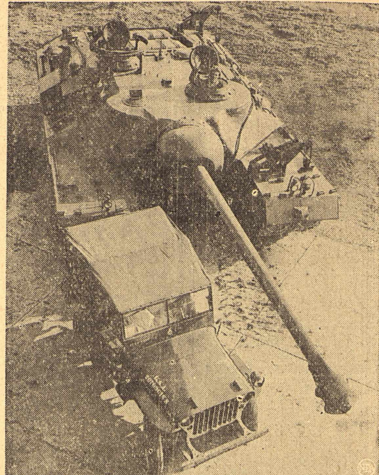
Heaviest vehicle ever built for the Army is the huge tank pictured above, contrasted in size with a jeep. The tank, designated T28, weighs nearly 100 tons and carries a 105-mm. cannon. Hitherto secret, the monster was displayed to 6000 industrialists attending the annual Army Ordnance Association meeting at Aberdeen, Md.
