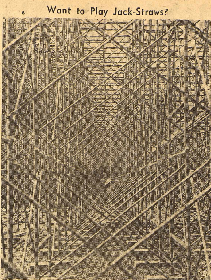
You'd need the hook of an electric crane to play with these "jack-straws," for they are made of steel tubing. This unusual picture shows the framework supporting the grandstand at the National Air Races at Cleveland, Ohio.
