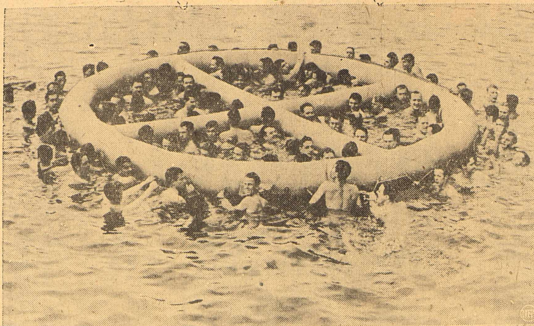
One hundred and four persons can be supported safely on the new type life raft pictured above being tried out at Dayton, Ohio. The huge "life preserver," 38 feet in circumference and weighing 79 pounds, was developed for the Army Air Forces at Wright Field, and will be used in major marine disasters.
