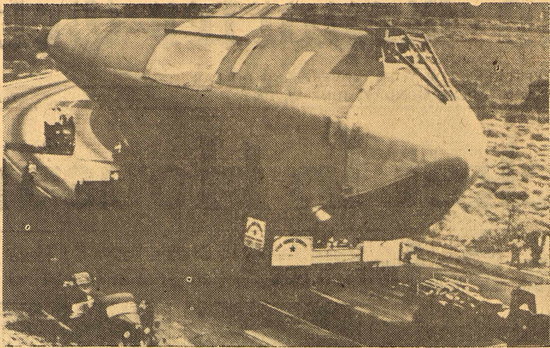
The gigantic 220-foot long fuselage of the Howard Hughes' flying boat crawls down the highway on truck dolly after leaving Culver City, Calif., on its way to Terminal Island, Calif., for assembly. The 28-mile trip was made at 29 miles per hour. Note the size of the man on top of the hull.
