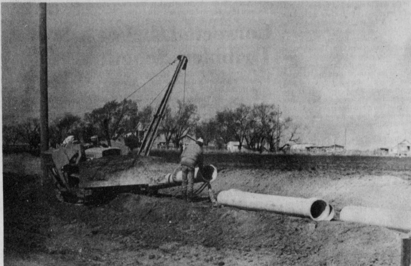
WORK CONTINUES on the water pipeline that will tie in with the Mackenzie water project. These workers are laying pipe west of Second Street. Operating the winch is Henry Martin and Jerry Powell is positioning the pipe to be connected with the previous section.
