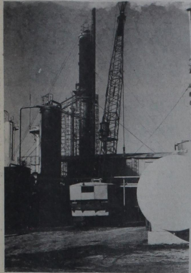
TO CLEAR THE AIR —The tall tower at the left of the crane pictured here was erected last week at Dimmitt's Western Ammonia plant. The 76 ft. structure is part of equipment being installed at the plant to remove the yellow coloring from the smoke emitted from the plant's smokestack. According to plant manager M. J. Reed, the equipment should be in operation at the plant sometime in March.
