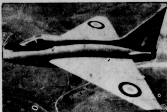
FLYING LABORATORY —Designed for high-speed aerodynamic research is this new delta-winged jet plane, shown being tested in England for the British Ministry of Supply. The single-seat craft is powered by a Rolls-Royce Nene turbojet engine. Performance details are secret.
