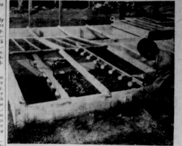
GIVE LIGHT AND SEEDLINGS WILL HUSTLE—Coddle your seedlings in electric hotbeds like these and you get your vegetables 10 days earlier, or your flower blossoms a month earlier, says Robert L. Zahour, Westinghouse engineer at Bloomfield, N. J. Here he looks over a set of three- by six-foot frames which are warmed by eight regular 25-watt incandescent light bulbs each.
