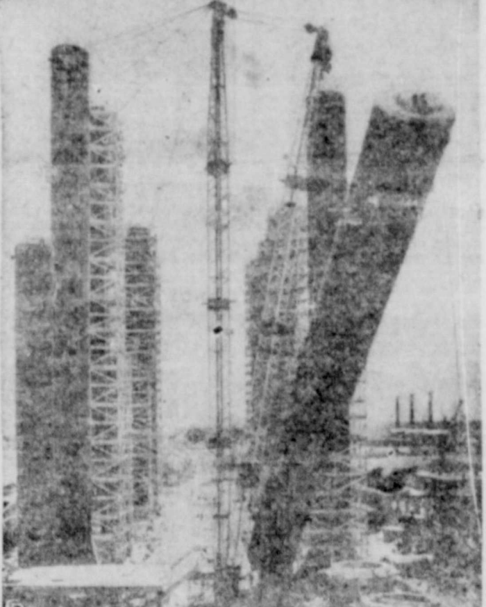
WORLD'S BIGGEST PLANT for the production of butadiene, chief ingredient of synthetic rubber, is being built on the Texas plains and will be operated by the oil industry—without profit. The towers, as high as 17-story buildings, were fabricated on the site and lifted into place by giant cranes. The plant will turn out 100,000 tons of butadiene a year, enough to fill one-seventh of war-time needs. (International)
