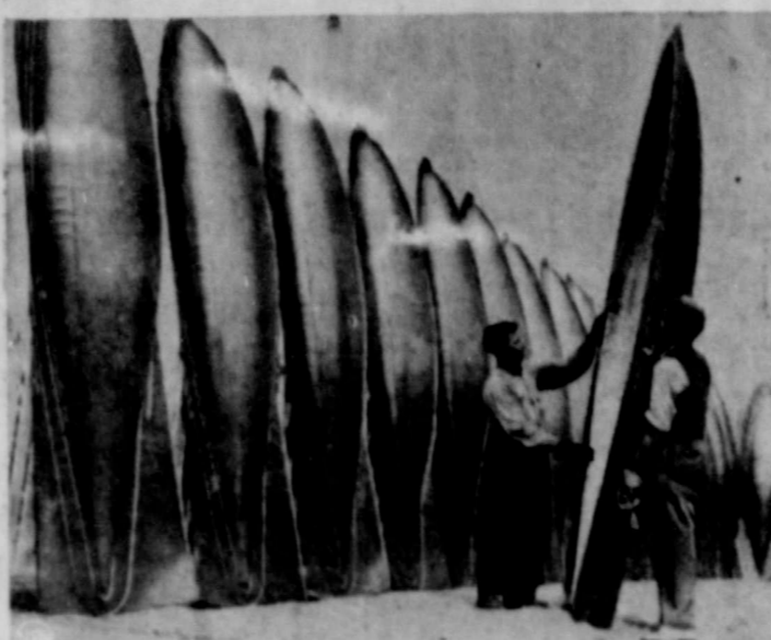
So that Lightnings can strike farther, the Lockheed P-38's now carry two droppable gas tanks under the center wing when going on long-range missions. The tear-drop tanks, bottom, are made in two sections, then welded together when attached to the P-38's.
