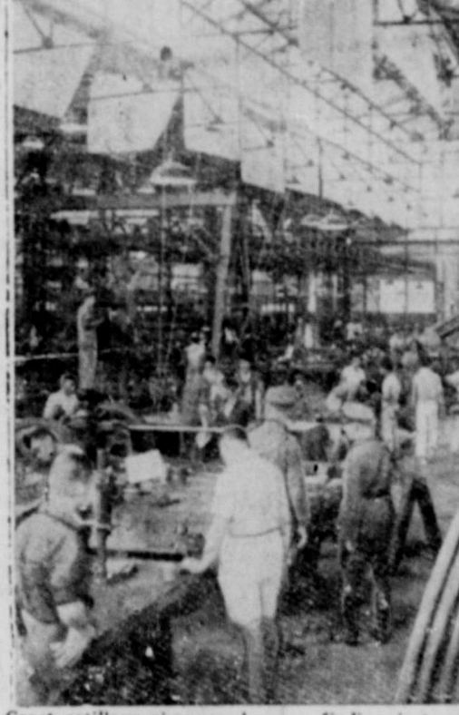
Coast artillery pieces and range finding instruments are assembled and repaired in this Army ordnance shop in Bandoeng, Java. In background is a standard Netherland Indies Army 8-centimeter anti-aircraft gun.
