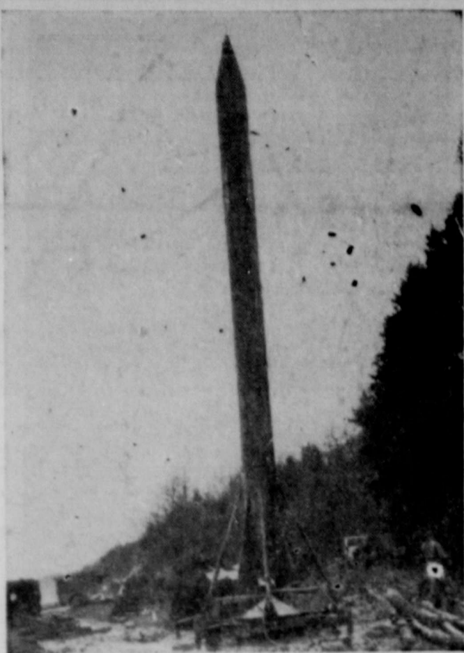
OVERSEAS GUARDIAN —Although it has been fired only in this country, as it was recently at a public shoot in New Mexico, the Army's 75-mile Corporal is deployed overseas. Here it rests in its light take-off pedestal in Germany, ready to be triggered for faster-than-sound flight if necessary.
