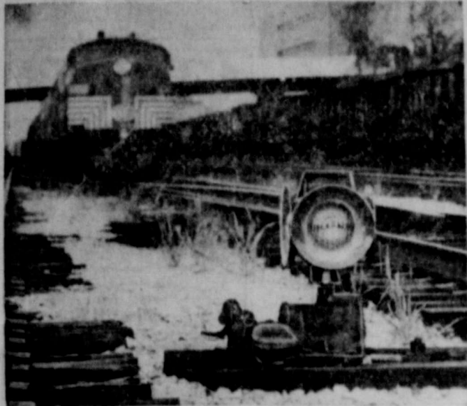
CLEAR TRACK TO NUCLEAR AGE—Switch lamp, in foreground, is a product of developments in nuclear physics. Krypton, a gas, reacts on the lining in the lamp and a glow results. The lamp has a potential life of 10 years without maintenance cost in its position along the New York Central's main line in Cleveland, Ohio. Both the Central and Pennsylvania railroads are installing the new lamps.
