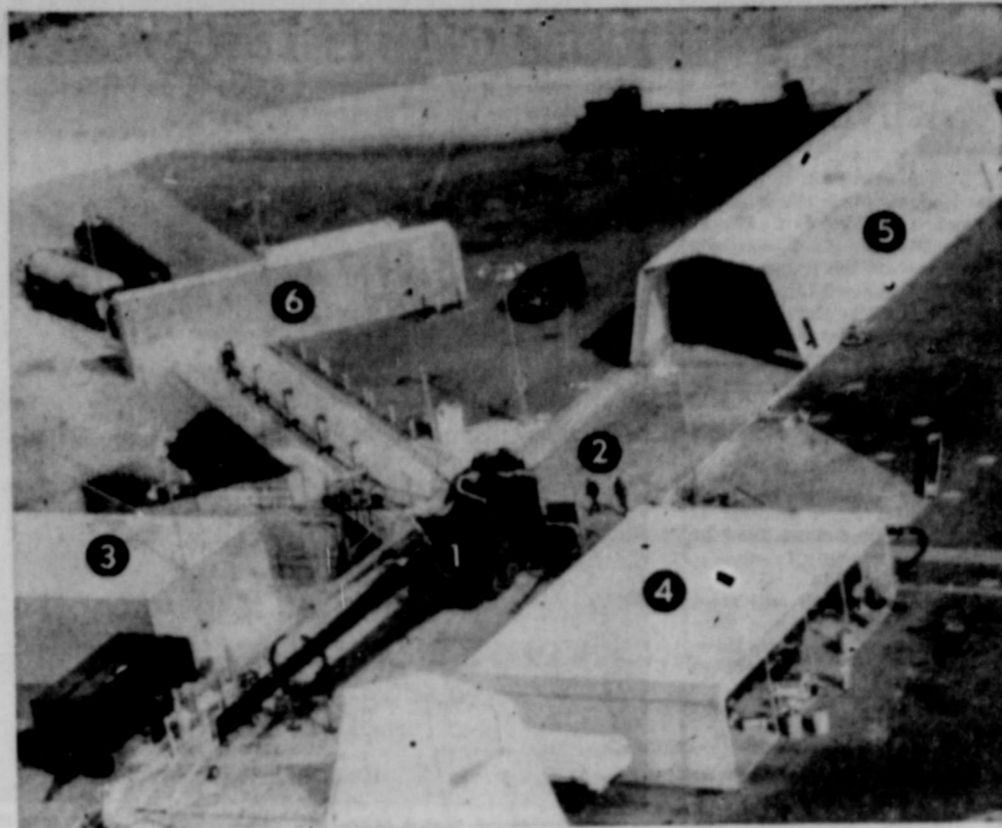
MISSILE LAUNCHING SITE —Here's the installation from which the first Thor intermediate range ballistic missile was launched at Uncle Sam's West Coast facility, Vandenberg Air Force Base, Calif. 1—Missile trailer serves also as crane to lift missile into place. 2—Launching pad. 3 and 4—Equipment buildings. 5—Shelter which rolls forward to cover missile area. 6—Protective barricade for trucks holding liquid fuels.
