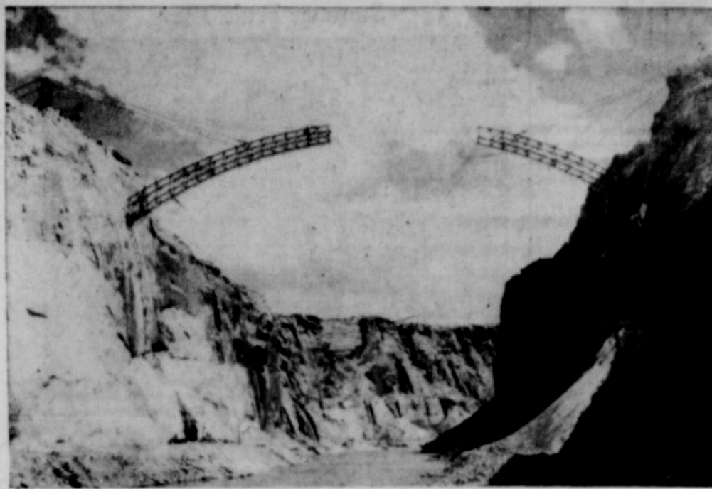
BRIDGE WILL LINK UTAH AND ARIZONA —The nation's highest and second longest steel arch bridge nears completion, 799 feet above the Colorado River near the Glen Canyon Dam site. The bridge will provide a new link between Utah and Arizona cities by January, 1959.
