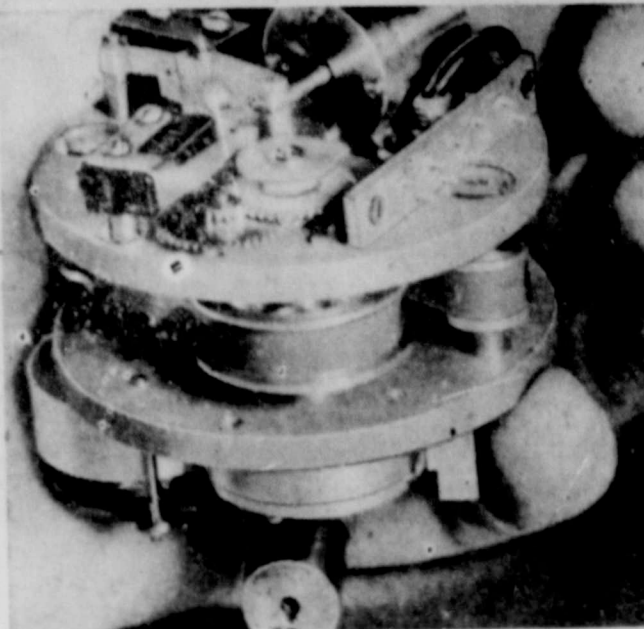
TINY TAPE RECORDER—It took 300 man hours to make this tiny tape recorder which was fitted into Explorer II, the Army's unsuccessful satellite. It was designed to store up information about cosmic rays, temperatures, meteorite bombardment and release it in five-second periods on signal from the ground. The completed assembly (a cover fits over it), built at University of Iowa, fits conveniently in a man's palm.
