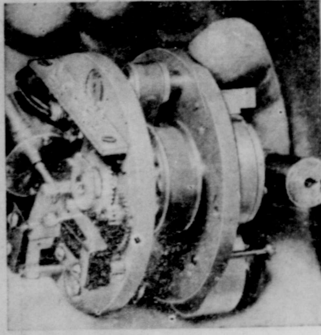
TINY TAPE RECORDER —It took 200 man hours to make this tiny tape recorder which was fitted into Explorer II, the Army's successful satellite. It was designed to store up information about cosmic rays, temperatures, meteorite bombardment and release it in five-second periods over the ground. The recorder is only about the size of a man's palm.
