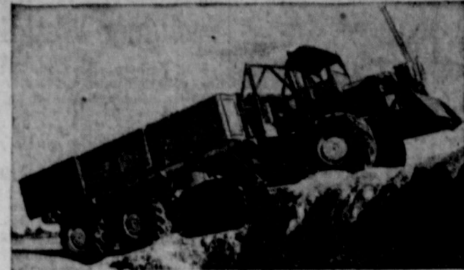
ROADLESS WONDER —No roads are needed for this vehicle. The Transporter, built by R. G. LeTourneau, Inc., of Longview, Tex., can haul a 70,000-pound cargo over steep embankments and ditches, through mud, sand or snow. Powerful electric motor is geared directly to each wheel to provide the Transporter with all-wheel drive.
