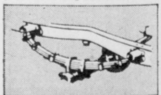
SIDE-MOUNTED REAR SPRINGS. Springs mounted to side of frame, typical of heavy duty construction.
