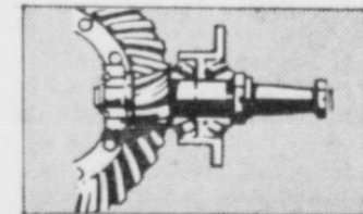
STRADDLE-MOUNTED PINION. Axle drive pinion held firmly by bearings on both sides of gear.
