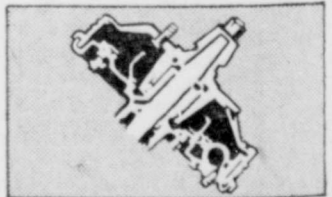
¾-FLOATING REAR AXLE. Typical of heavy truck design; axle shaft supports, axle housing carries the load.
