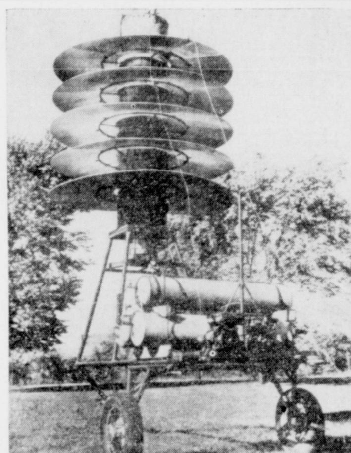
GOOD NEWS FOR FARMERS—This machine, developed by Michigan State College of Agriculture engineers, is said to protect an acre of crops from frost damage. The apparatus burns oil and generates infra-red rays which do the work. It is reported to be economical to use and not costly to build.
