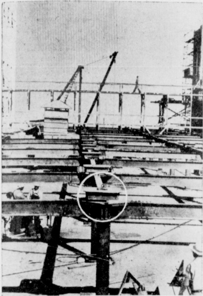
IN ANTICIPATION—Shown in the circle is a new earthquake roller bearing, one of 65 sets which will provide a rolling foundation for the three-story addition to a Los Angeles building. The entire addition will be able to shift six inches.
