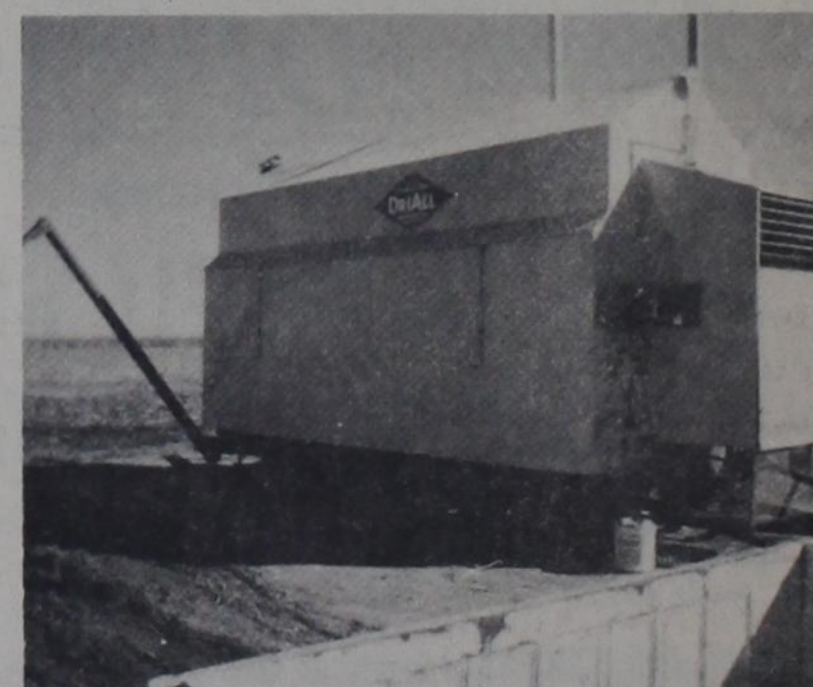
PORTABLE CONTINUOUS FLOW CORN DRYER ON THE FARM OF JAMES WELCH
