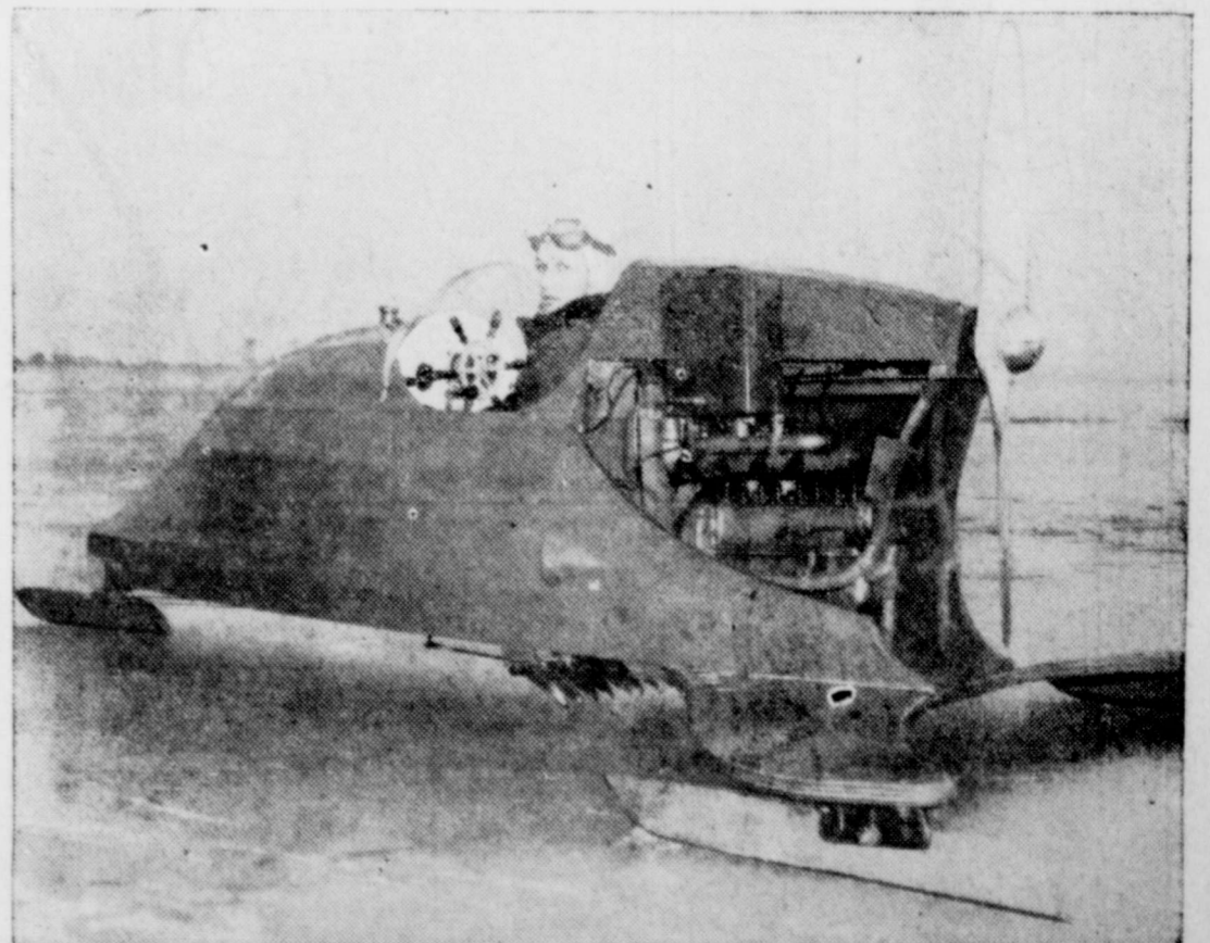
HOMEMADE ICE BOAT —Steve Noawojki of Chicago, a former Seabee, sits in ice boat he constructed. The craft, propelled by converted motorcycle engine, can attain speed of 135 m.p.h.
