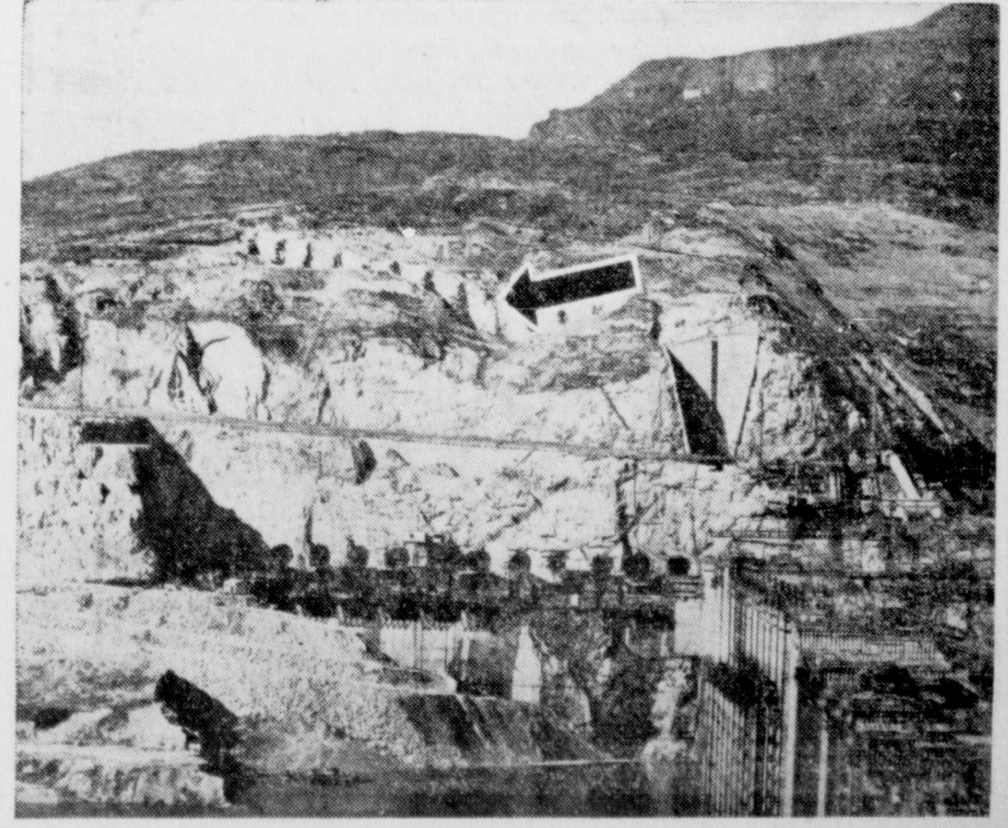
RESEMBLING PRIMITIVE CAVES , these tunnels which emerge half way up the hill, indicated by arrow, have been driven through barrier of granite at Grand Coulee Dam, Wash. World's largest pumps, to be installed in tunnel entrances, will force water from Lake Roosevelt, foreground, through 12-foot steel pipes installed in the bores. Pipes will convey water two miles to reservoir.
